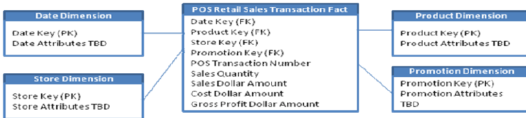
Measured facts in the retail sales schema
